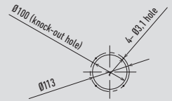
Fresh air intake duct connection port (detail)
