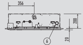
Fresh air intake duct connection port (detail)
