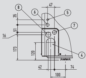
View Z
