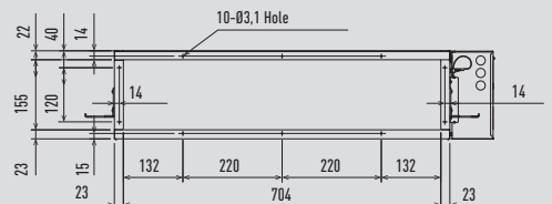
View A Frame filter uninstalled
