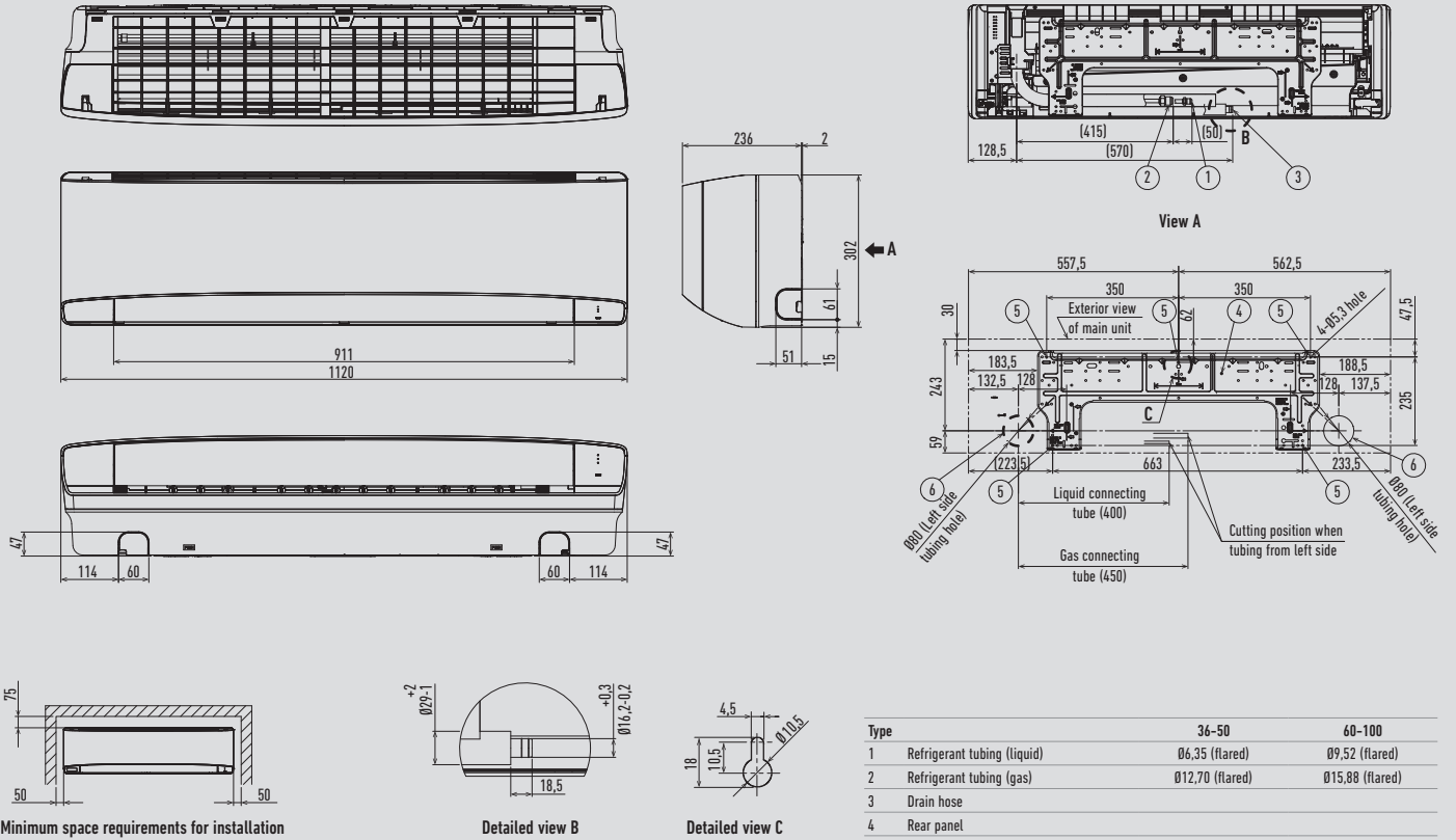
Minimum space requirements for installation
