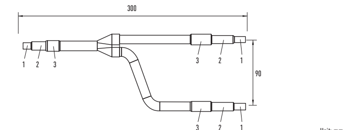
Liquid tubing
